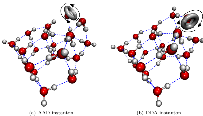
Figure 6.2: Conformed snapshots of the considered 20mer tunnelling paths. The structures were obtained using the TTM3-F potential.
