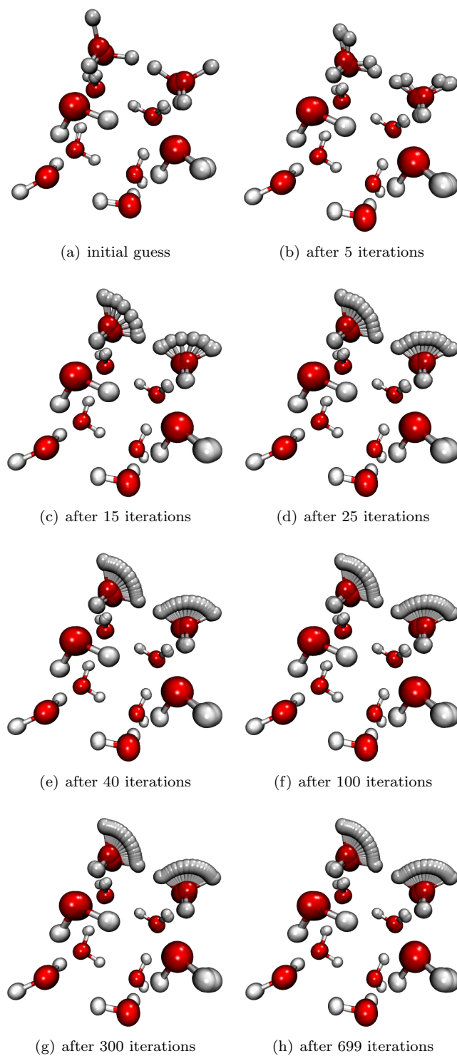
Figure 3.1: Convergence of a water decamer instanton with 256 beads at \hbar\beta = 20000 a.u.. After 699 iterations convergence to \varepsilon = 10^{-5} a.u. was achieved.
