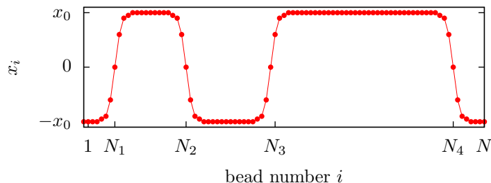
Figure 2.4: A 4-kink trajectory in the double well system V(x) = \lambda(x^2 - x_0^2)^2 starting and ending at -x_0 . The kinks may be distinguished from one another by the number of the central bead N_1, N_2, N_3, N_4 . (Based on Richardson and Althorpe [12])
