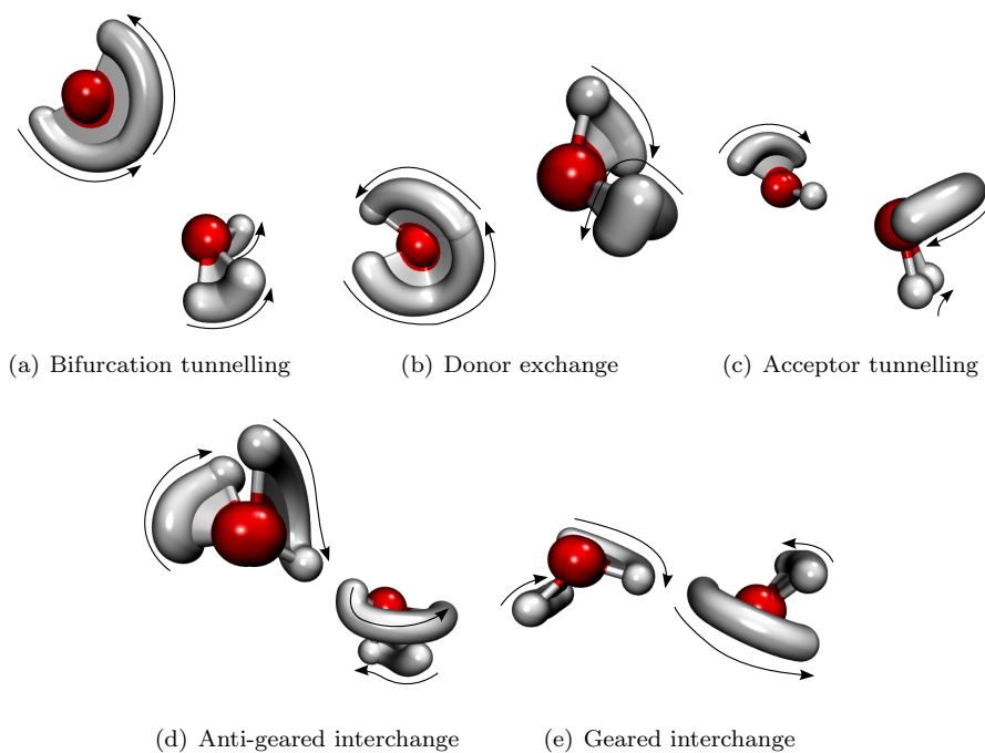
Figure 5.2: Conflated snapshots of the dimer instanton tunneling paths obtained using the TTM3-F potential.
